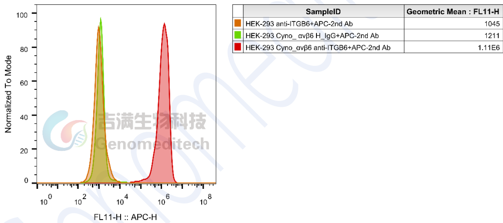
Fig 3. Cynomolgus_αVβ6 HEK-293 Cell Line (Genomeditech / GM-C28127) 使用: Anti-ITGB6 hIgG1 Antibody(SGN-B6A) (Genomeditech / GM-81622AB) 抗体流式验证结果
