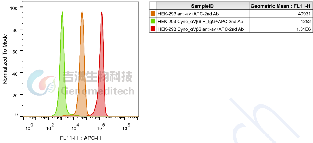
Fig 2. Cynomolgus_αVβ6 HEK-293 Cell Line (Genomeditech / GM-C28127) 使用: Anti-αV(Abituzumab)hIgG2 Antibody (Genomeditech / GM-49298AB) 抗体流式验证结果
